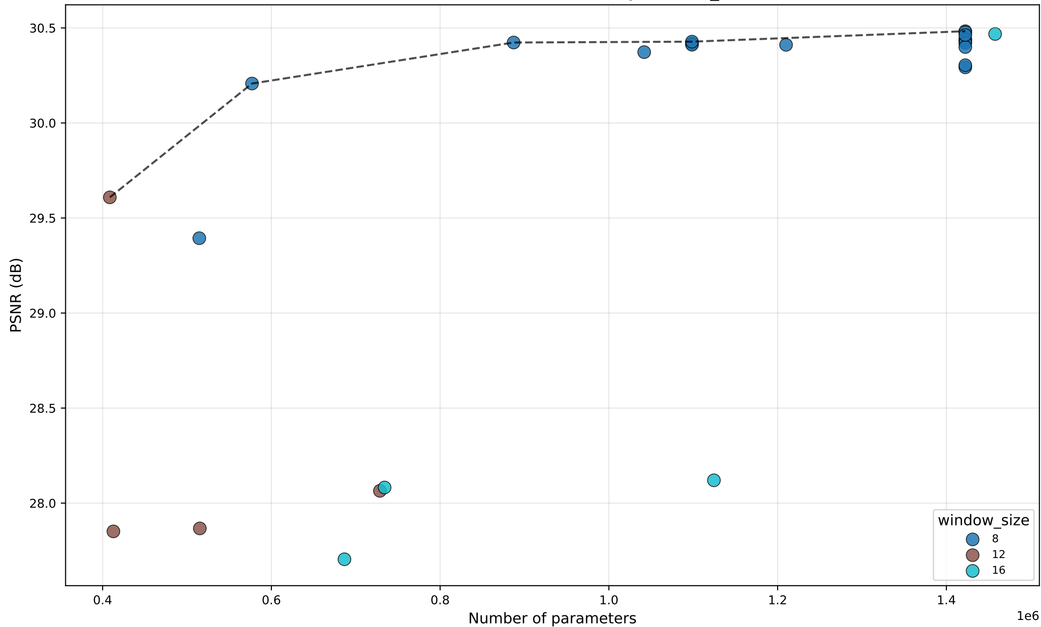
PSNR vs #Params — SwinT — by window_size
